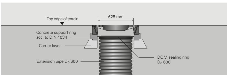
Standard cover (625 mm)
